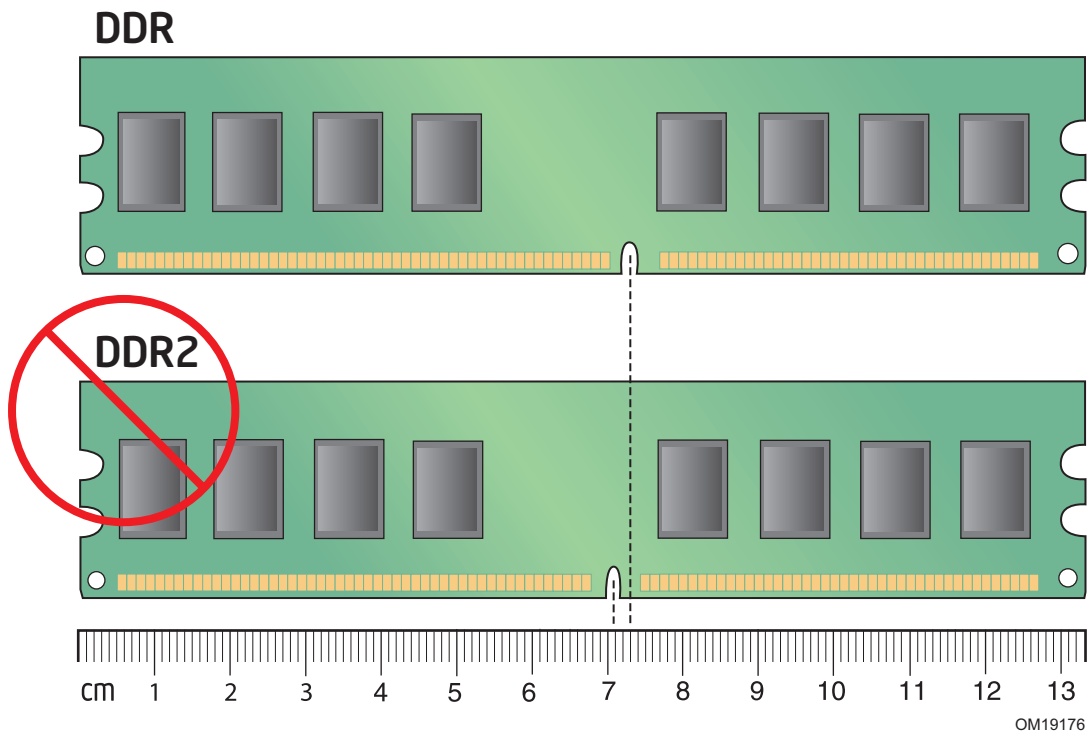
Figure 14. Use DDR DIMMs
